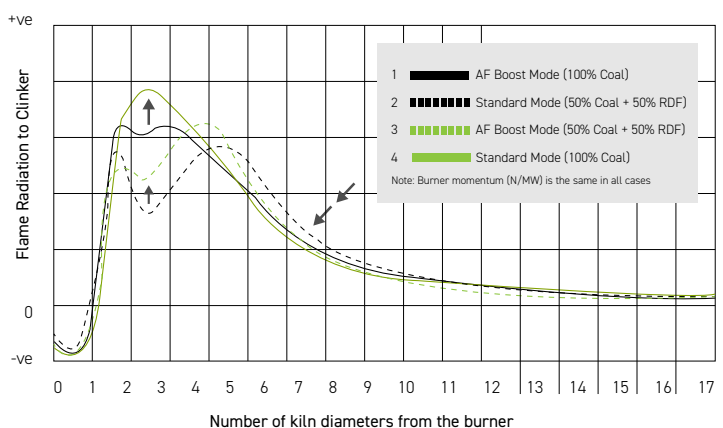
Flame Radiation to Clinker for Coal and RDF
